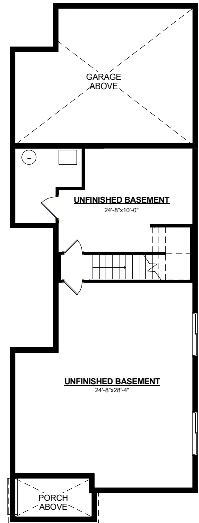
BASEMENT LEVEL FLOOR PLAN 1131 SF
