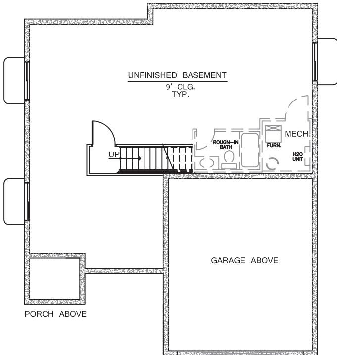
BASEMENT LEVEL FLOOR PLAN 1,042 Sq Ft
