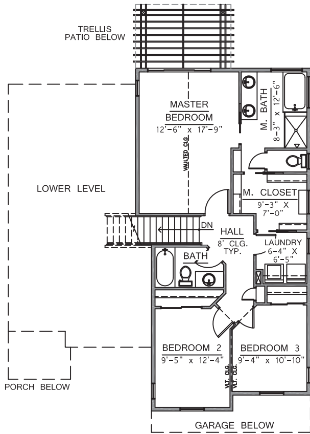
UPPER LEVEL FLOOR PLAN 902 Sq Ft
