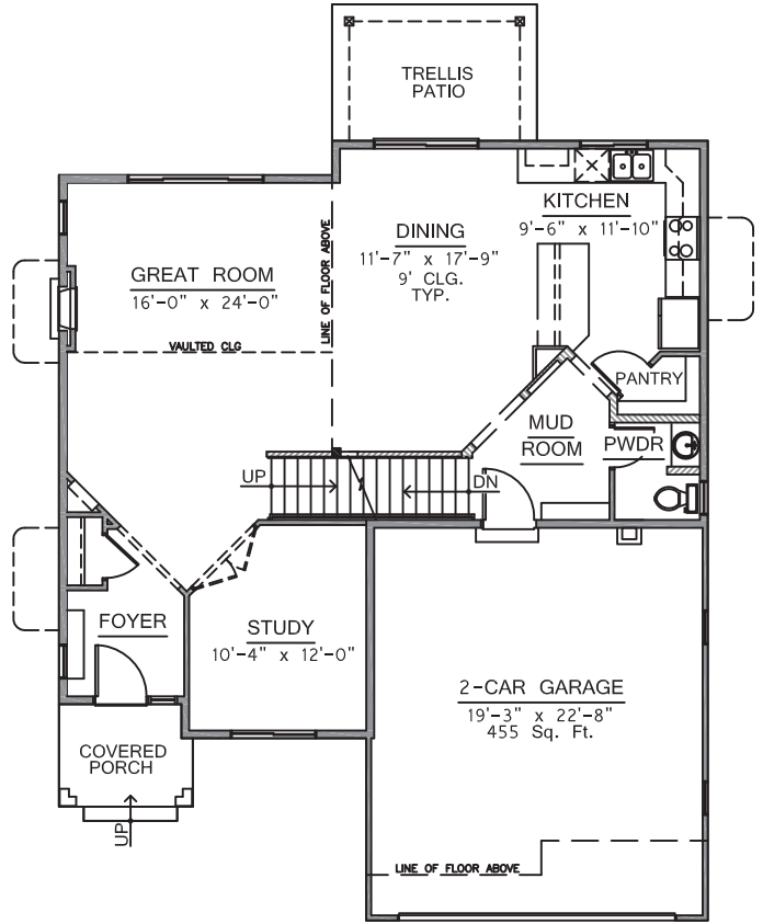
MAIN LEVEL FLOOR PLAN 1,039 Sq Ft
