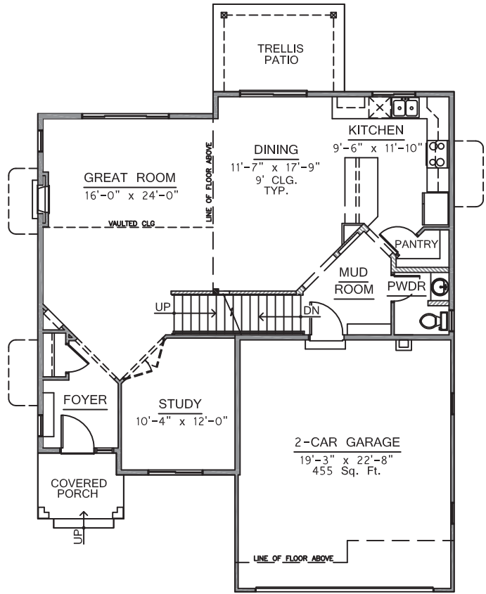
MAIN LEVEL FLOOR PLAN 1069 Sq Ft
